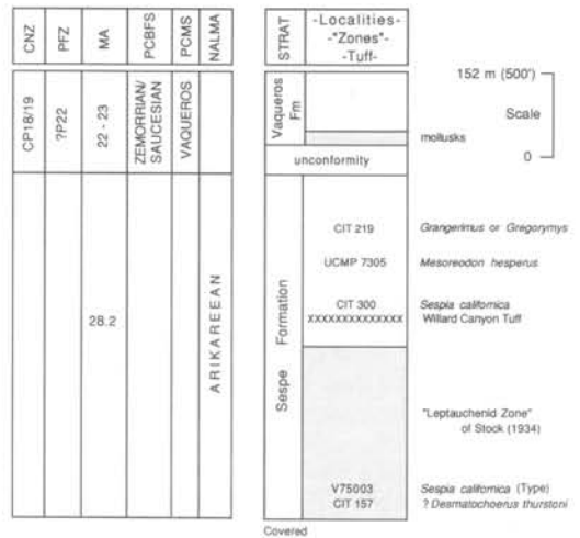
Figure 2. Generalized stratigraphic column and correlation chart for the Sespe Formation, South Mountain, California. Certain localities and taxa with less precise stratigraphic positions are not plotted; see faunal list (Table 3) for additional paleontologic and stratigraphic data. Abbreviations are as follows: NALMA, North American Land Mammal Age; PCMS, Pacific Coast Molluscan Stage; PCBFS; Pacific Coast Benthic Foraminiferal Stage; MA, megannum; PFZ, Planktic Foraminiferal Zone; CNZ, Calcareous Nannofossil Zone. Data from Stock (1930, 1934, unpublished), Wilson (1949), McDougall (1983), Poore and Bukry (1983), Yeats (1987), Turner (1970), and this paper.
